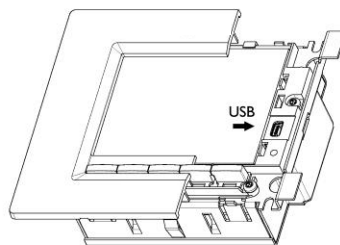
TSW9500 front view removable front plate
