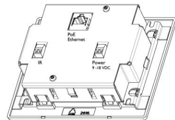
TSW9500 back view connections
